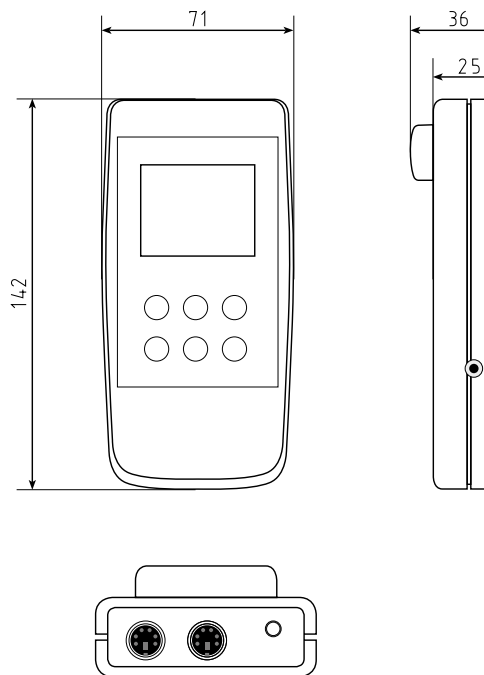
Digital indicator CPH6200-S2
