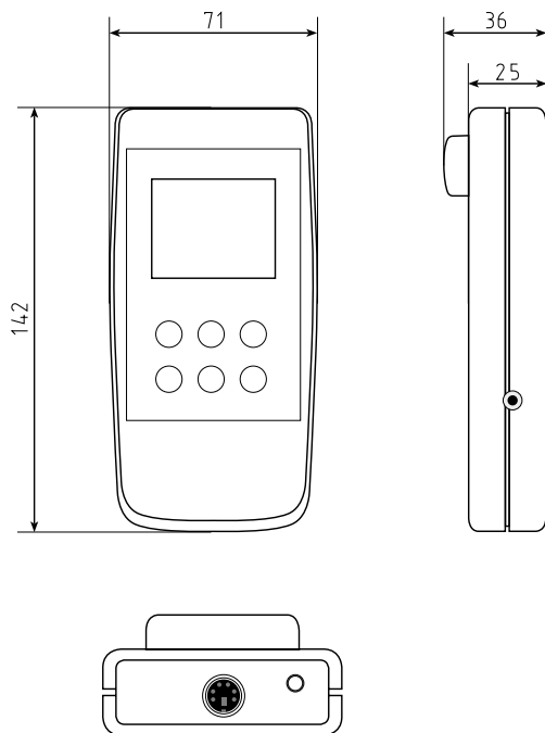
Reference pressure sensor CPT6200
