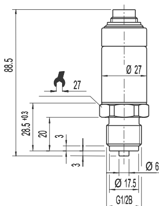
Reference pressure sensor CPT6200
